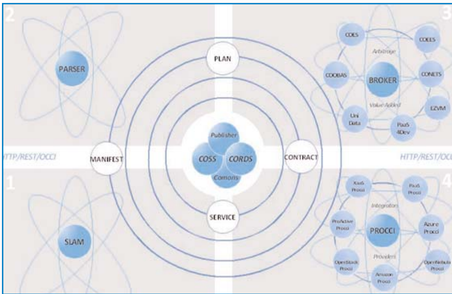
FIGURE 1. ACCORDS PLATFORM
